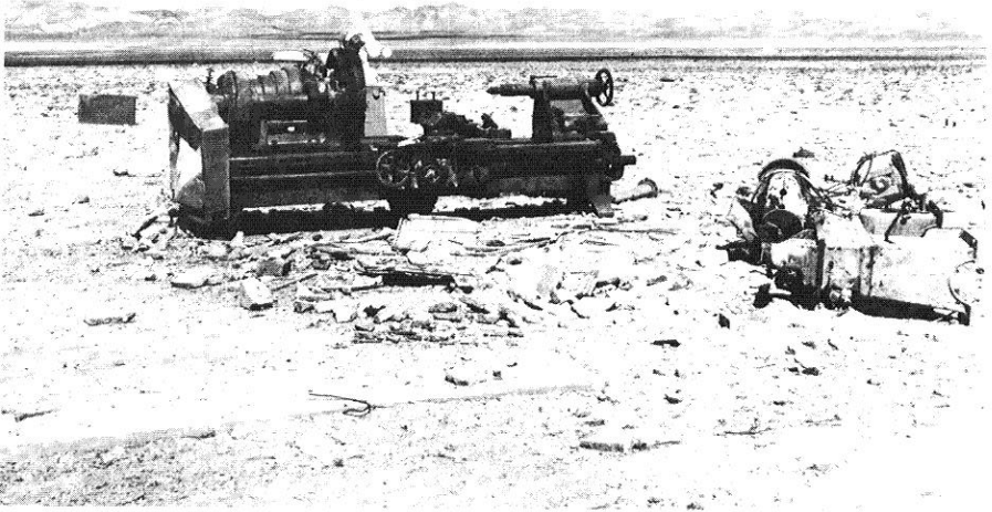
Figure 5.129a. Machine tools after a nuclear explosion (10 psi peak overpressure).
