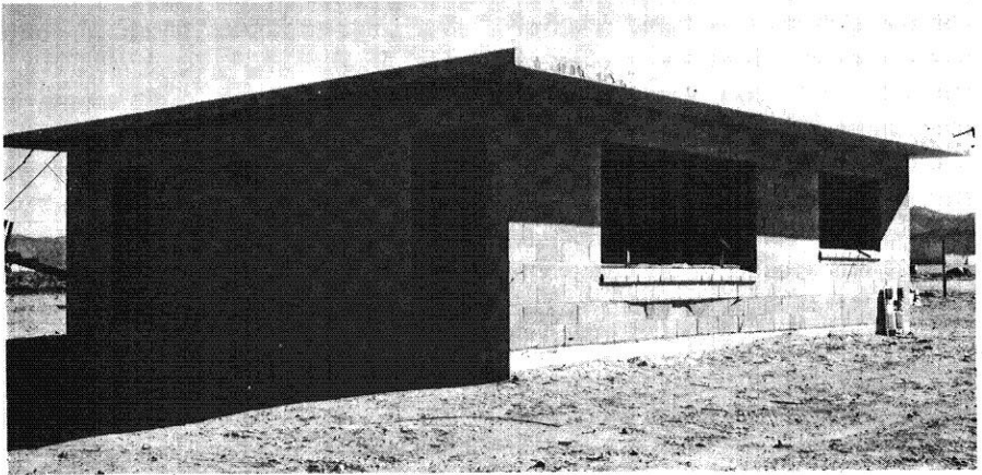
Figure 5.77. Reinforced masonry-block house after a nuclear explosion (5 psi peak overpressure).
