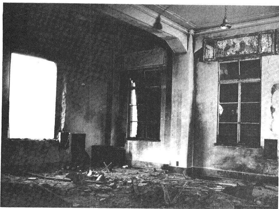
Figure 7.66. Fire shutters in building blown in or damaged by the blast; shutter at center probably blown outward by blast passing through building (0.57 mile from ground zero at Hiroshima).
