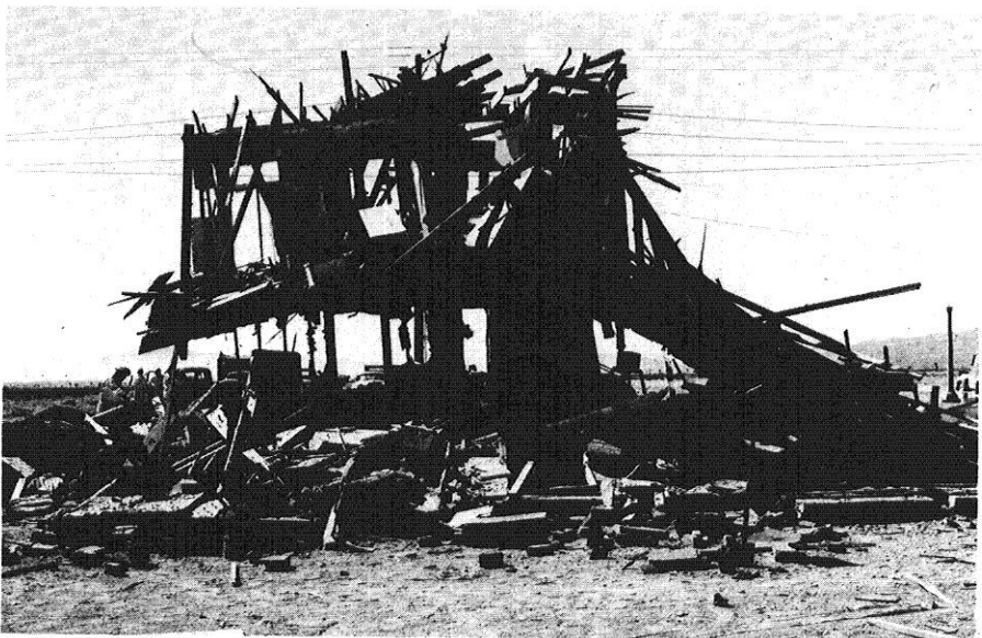
Figure 5.67. Unreinforced brick house after a nuclear explosion (5 psi peak overpressure).
