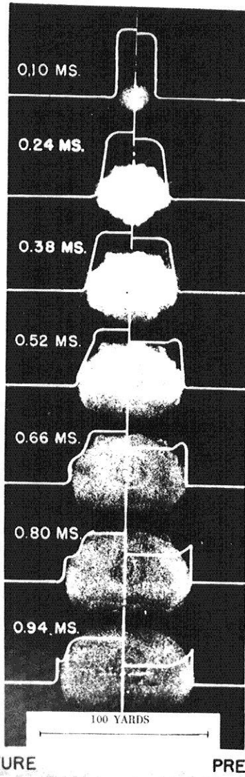
Figure 2.118. Variation of temperature and pressure in the fireball. (Times and dimensions apply to a 20-kiloton air burst.)
