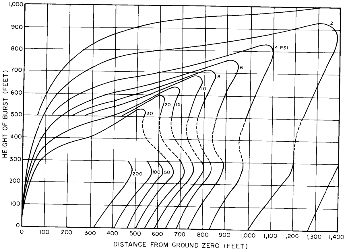
Figure 3.75. Horizontal component of peak dynamic pressure for 1-kiloton burst.
