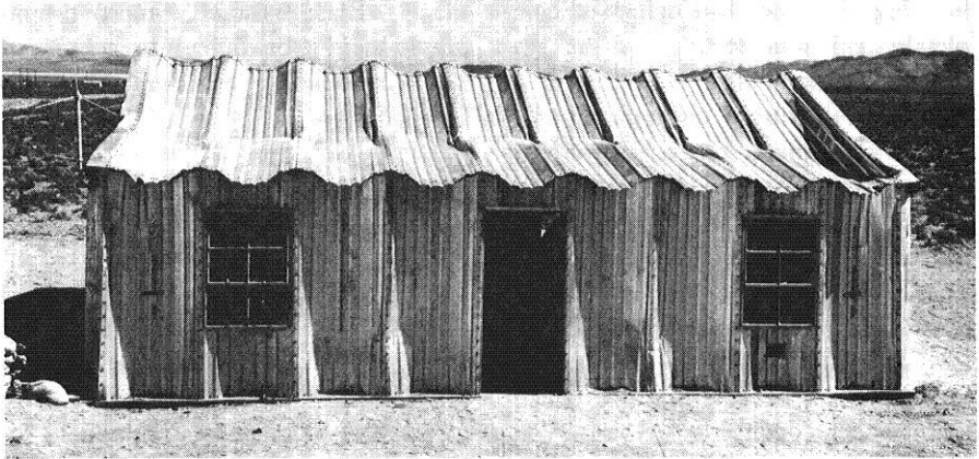
Figure 5.44. Self-framing corrugated steel panel building after a nuclear explosion (3.1 psi peak overpressure).
