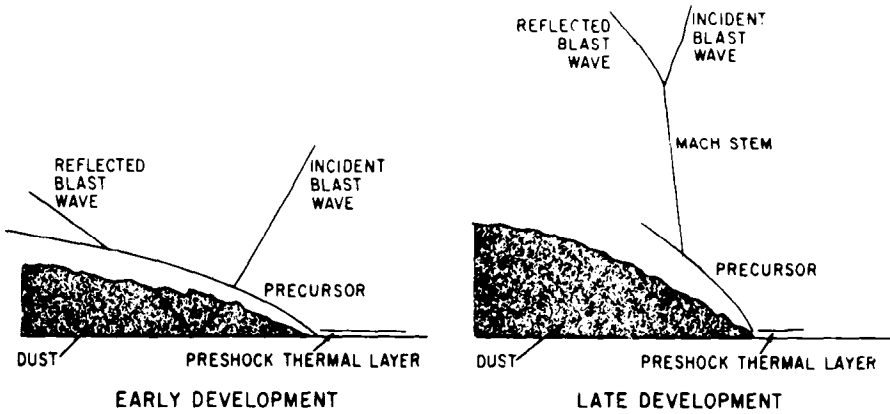
Figure 3.81. Precursor characteristics.
