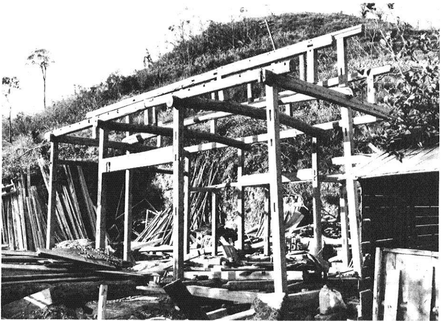
Figure 5.52. Upper photo; Wood-frame building; 1.0 mile from ground zero at Hiroshima. Lower photo: Frame of residence under construction, showing small tenons.
