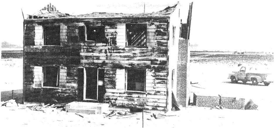
Figure 5.64. Strengthened wood-frame house after a nuclear explosion (4 psi peak overpressure).
