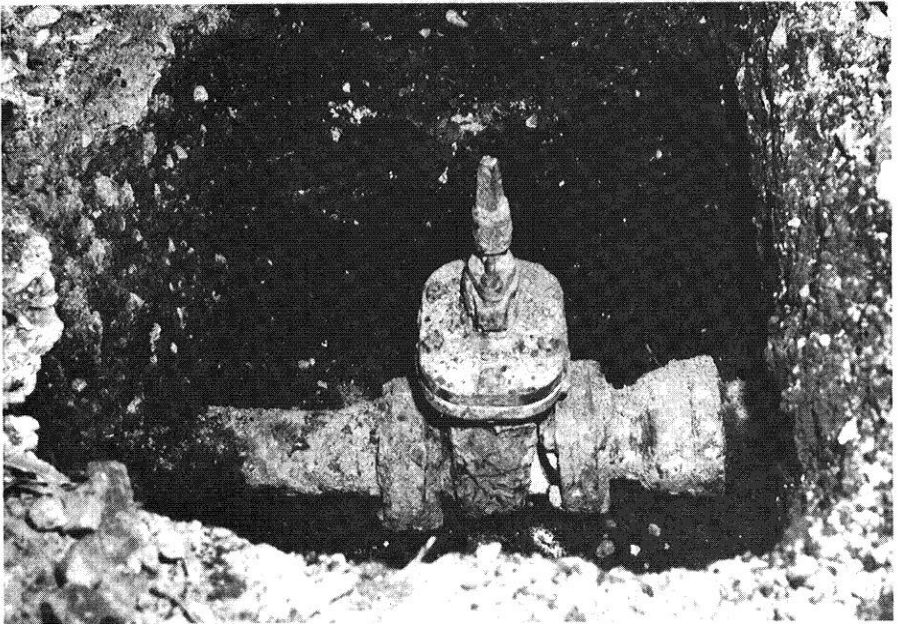
Figure 5.106a. Four-inch gate valve in water main broken by debris from brick wall (0.23 mile from ground zero at Hiroshima).
